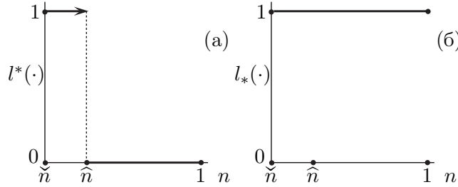
Рис. 22. Графики функций (а) l^*(n) = \min_{y \in Y} \tau_{y^*}^{\tilde{\xi}}(\vartheta(n)) , n \in [0, 1] ; (б) l_*(n) = \max_{y \in Y} \tau_y^{\tilde{\xi}^*}(\vartheta(n)) , n \in [0, 1] , Y = X .
